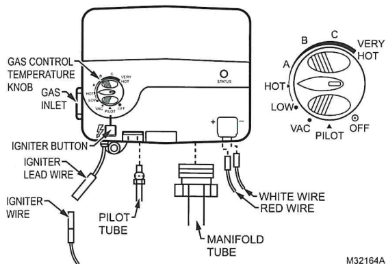
Fig. 2. Gas Control Valve/Thermostat
